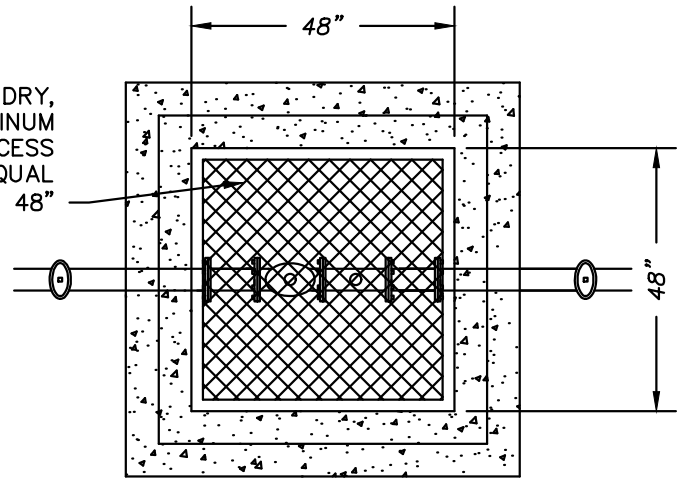
ACCESS HATCH NTS
