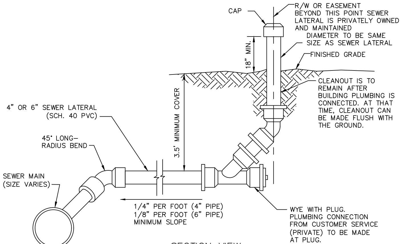
SECTION VIEW NTS
