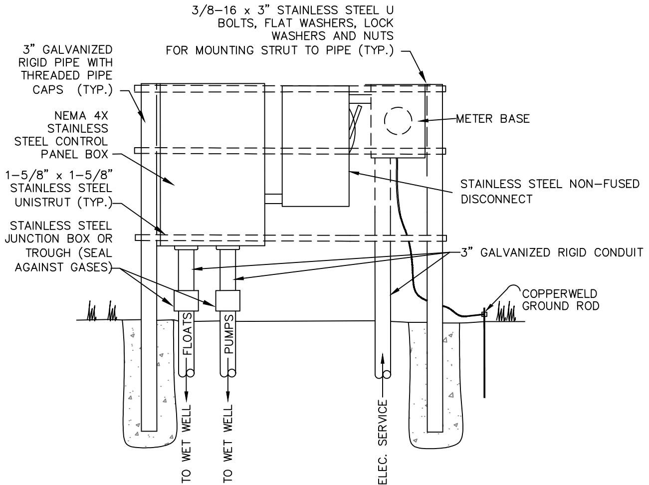
ELEVATION NTS
