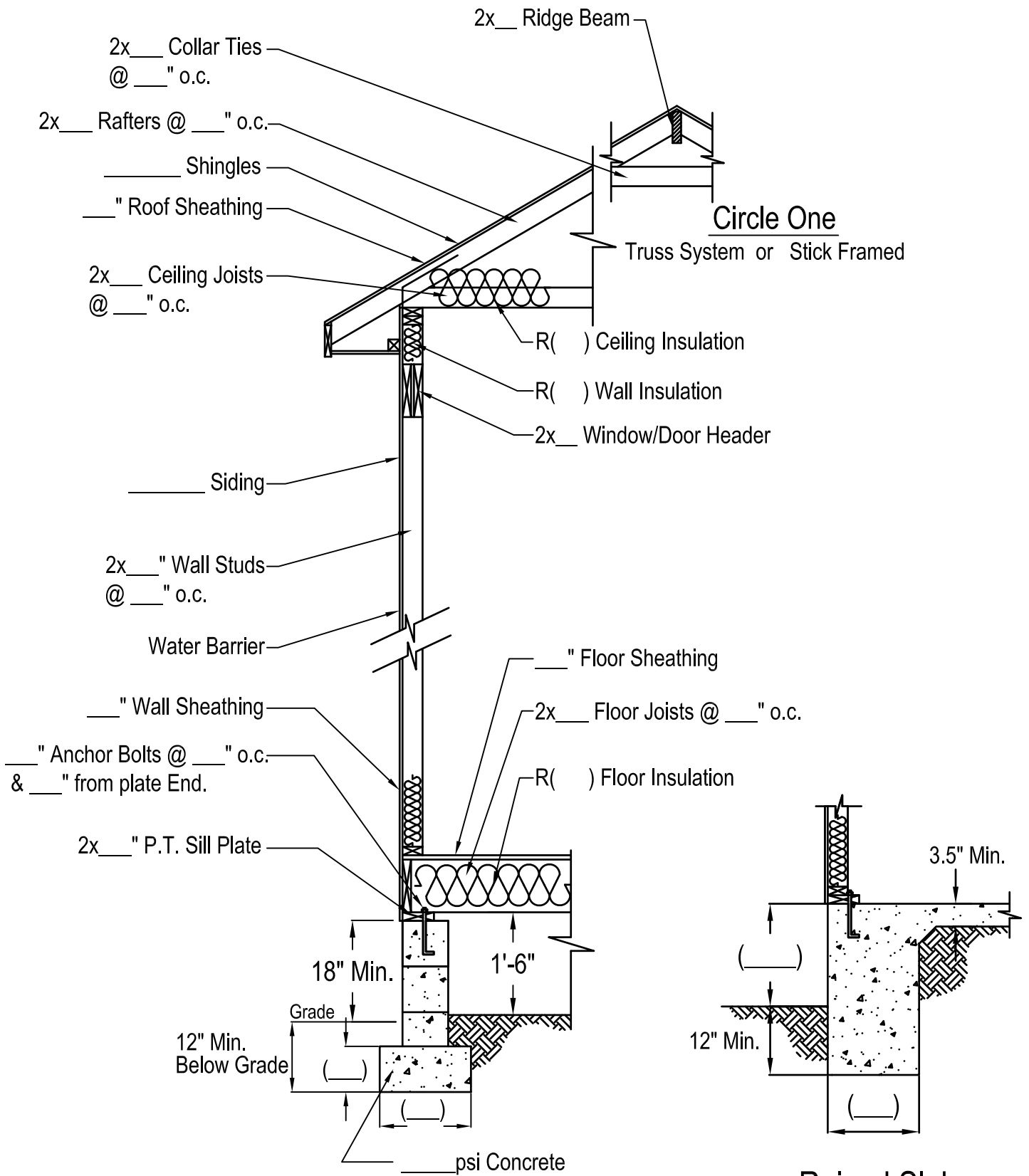
Raised Slab Foundation
